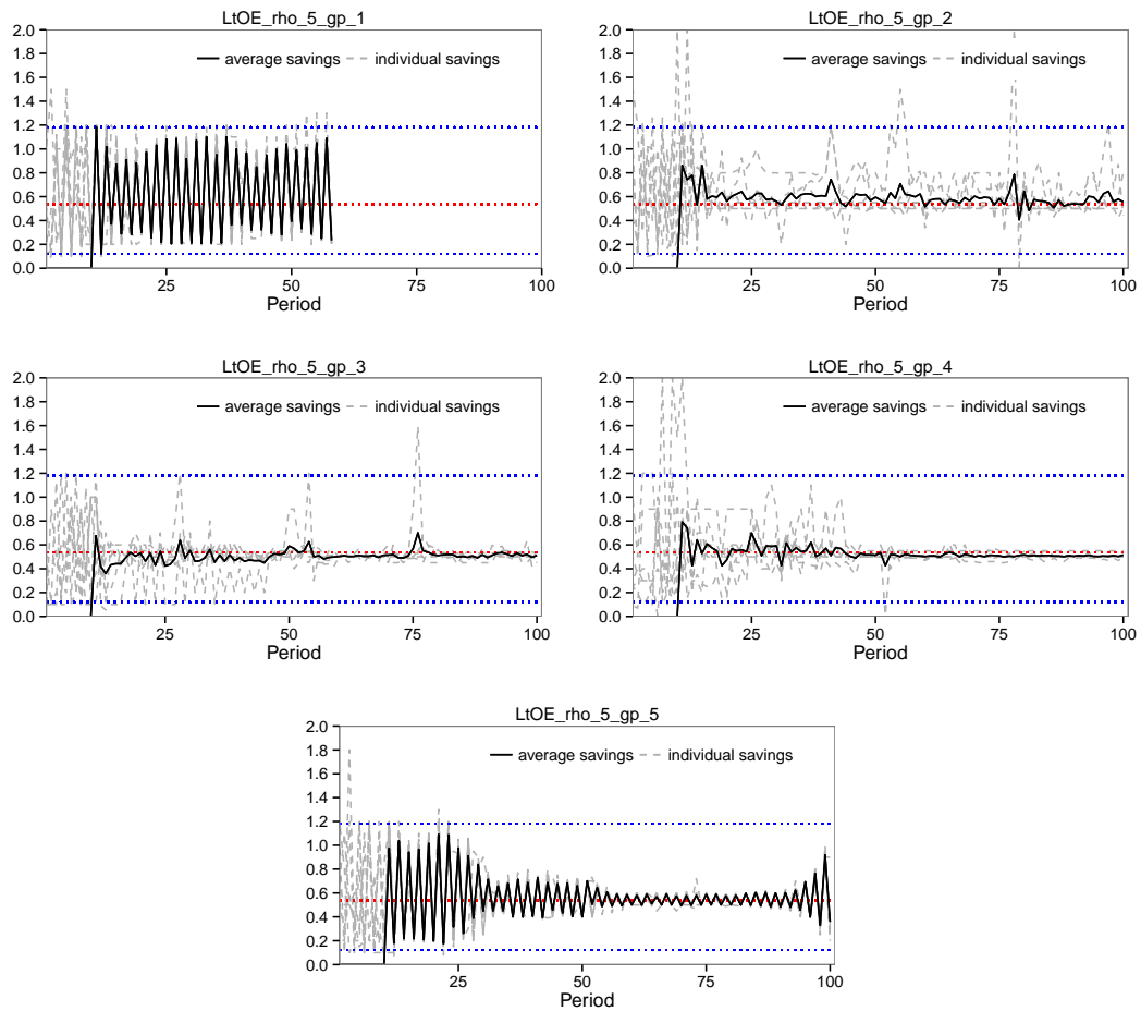
Figure 18: \rho_2 = 5 (2-cycle) with training . N.B.: a computer crashed at period 58 in group 1.
