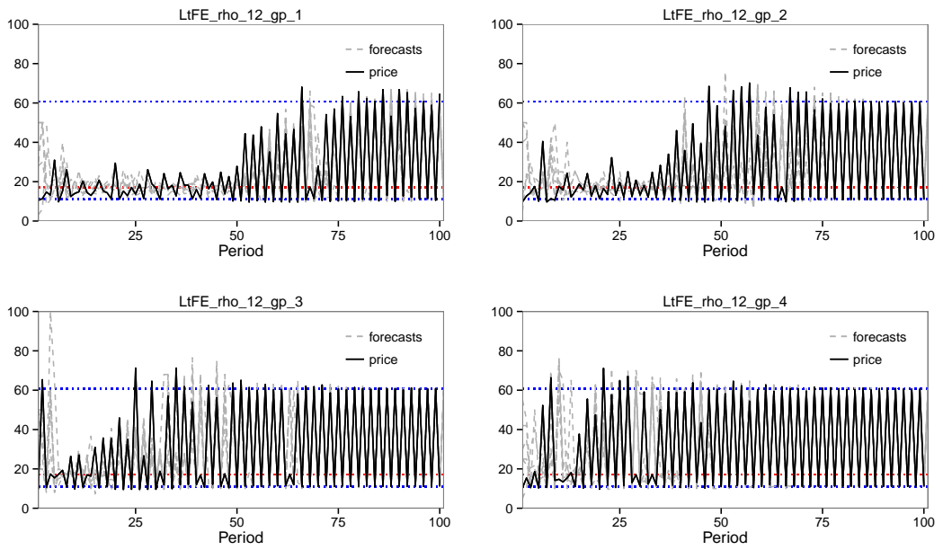
Figure 14: \rho_2 = 12 (chaotic dynamics)
