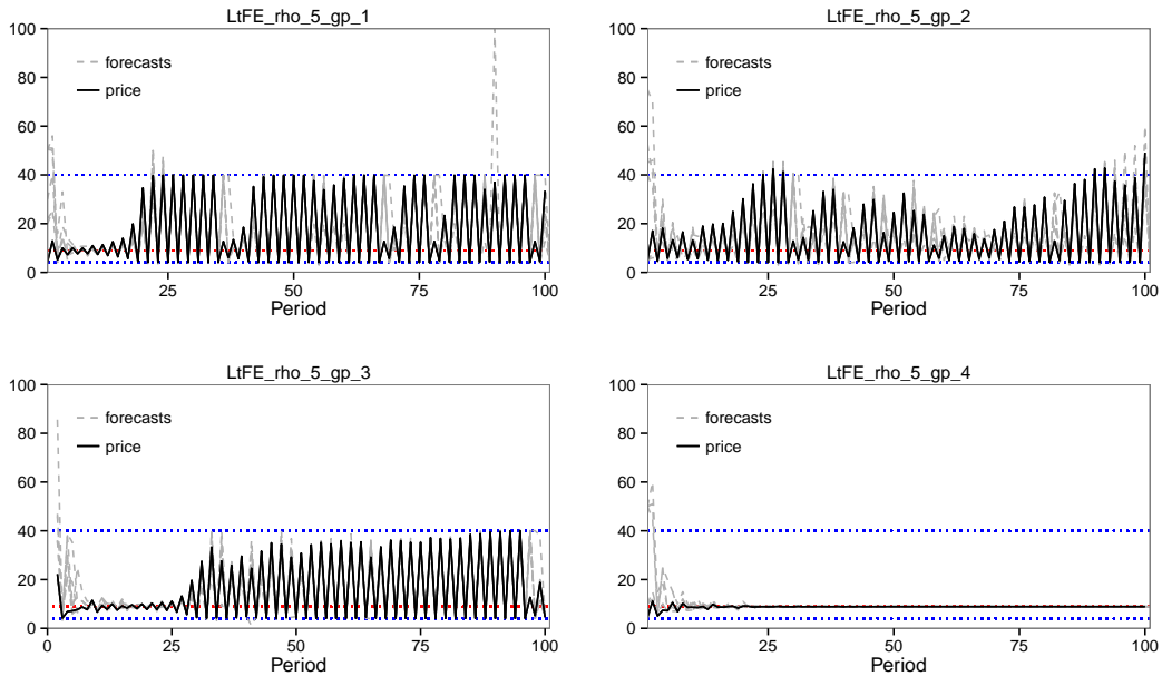
Figure 12: \rho_2 = 5 (2-cycle)
