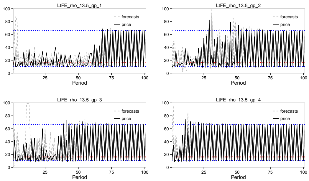
Figure 15: \rho_2 = 13.5 (3-cycle)
