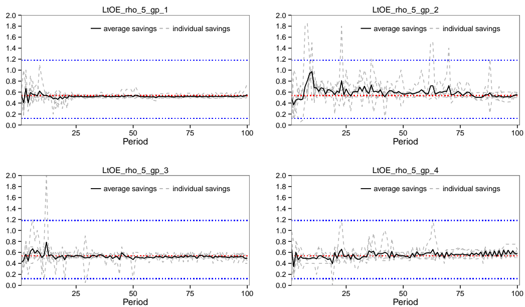
Figure 17: \rho_2 = 5 (2-cycle)
