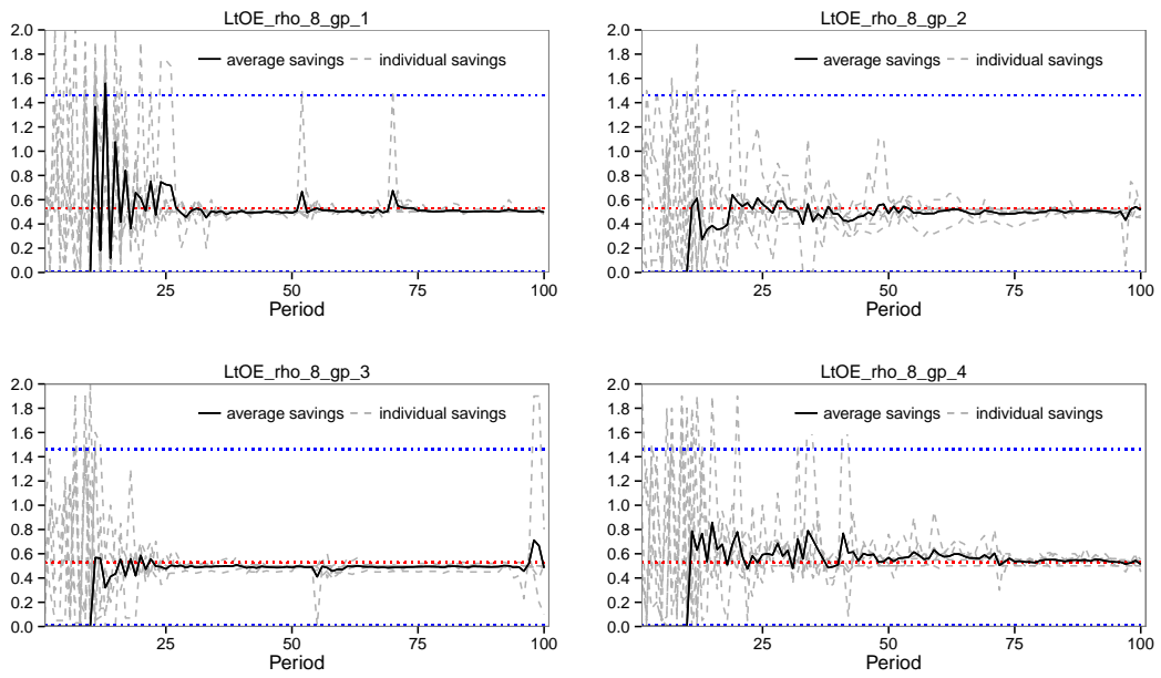
Figure 20: \rho_2 = 8 (32-cycle) with training
